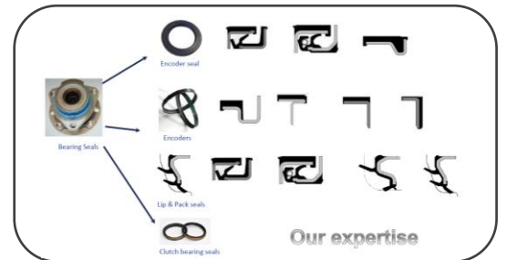
Hub Bearing Seals
