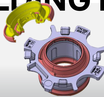
Static sealings overmolded on Metal-plastic insert
