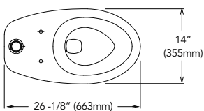
12" rough-in dimensions
