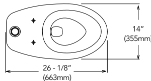
12" rough-in dimensions
