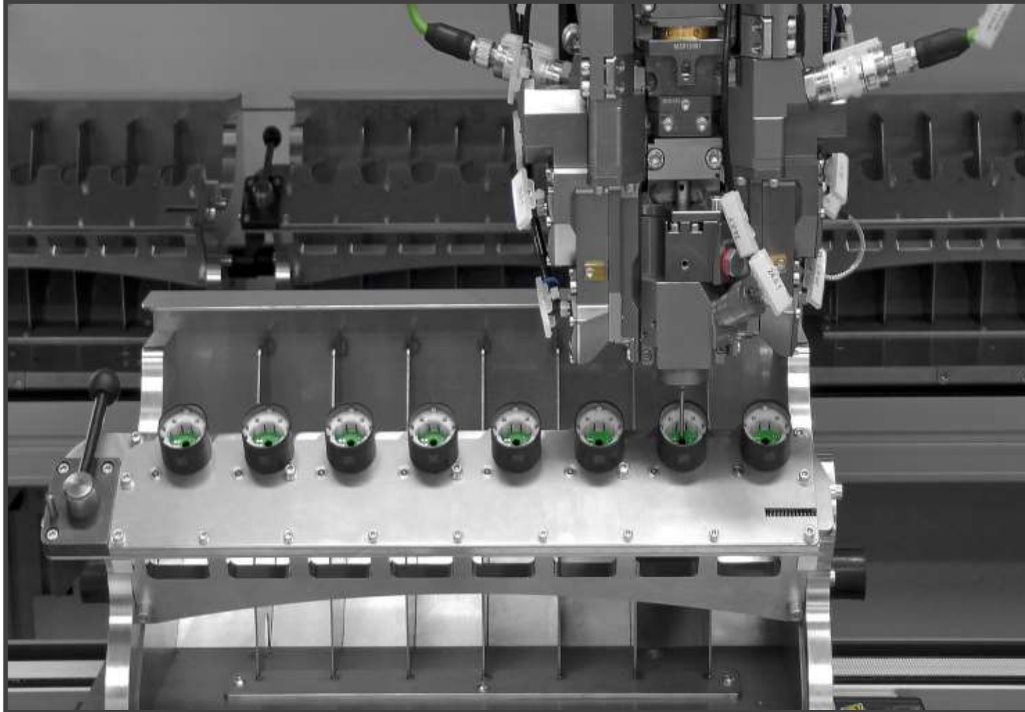
Automated Potting
