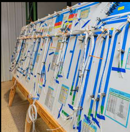
Connector and Wire Harness Assembly
