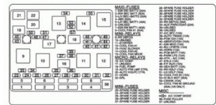
Fuse Block - Underhood Label
