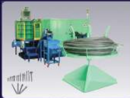
BOLT FORMER
