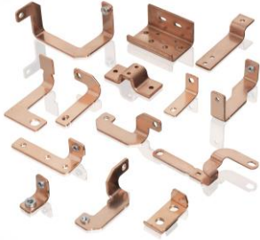
High current, thick copper battery busbars with PEMnut fasteners
