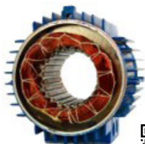
Insertion Winding
