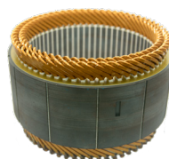
Hairpin Winding
