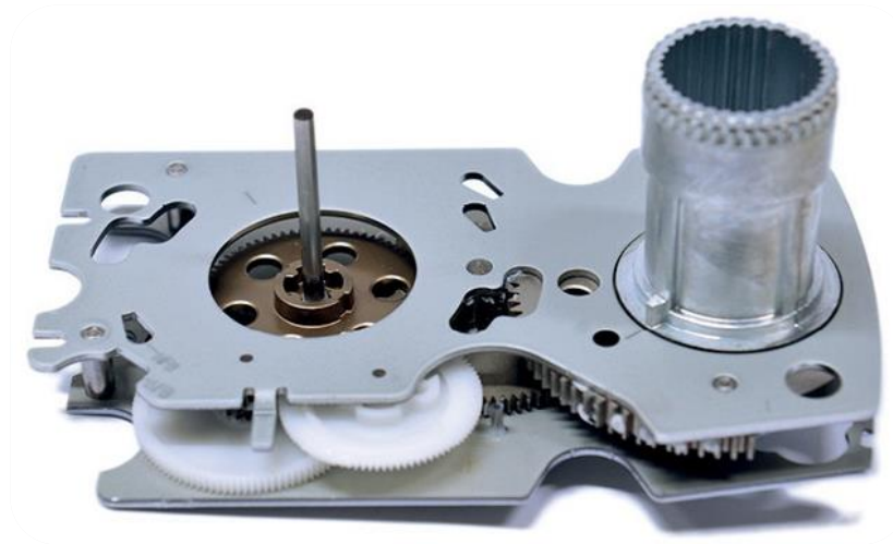
Gearbox
